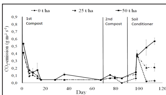
Figure 2. \text{CO}_2 emissions under 600 mg / L irrigation with different compost doses
