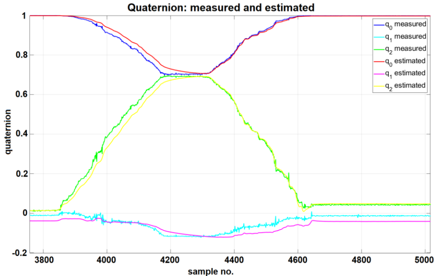
Figure 6 Quaternion filtration
