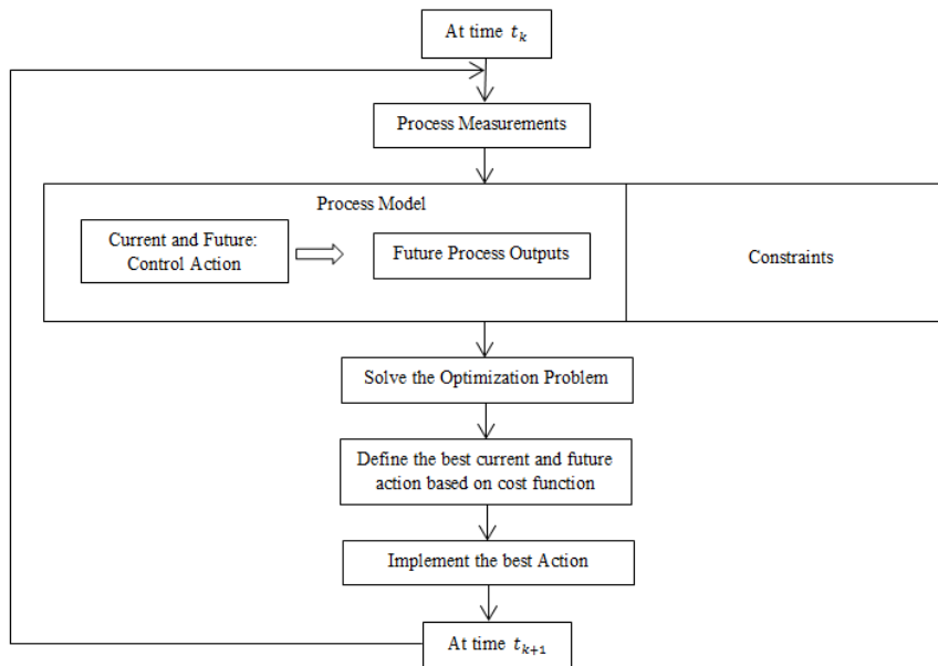
Figure 5 MPC Control Algorithm
