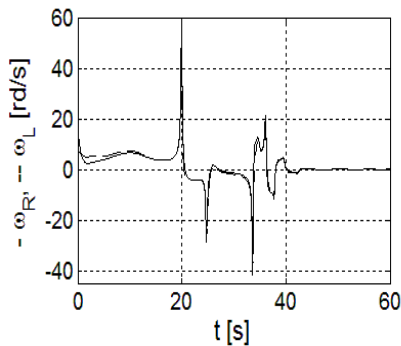
Figure 10a Wheel controls - simulation
