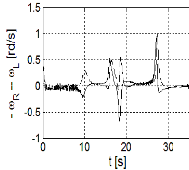
Figure 5b Platform controls – experiment
