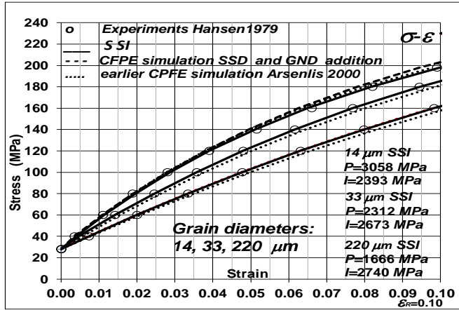
Figure 7 Stress-strain curves for average grain diameters of 14, 33 and 220 μm
