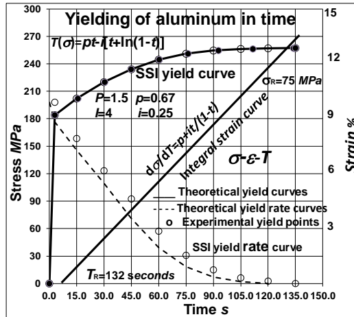
Figure 8 Stress and strain measurements on aluminium specimens in time
