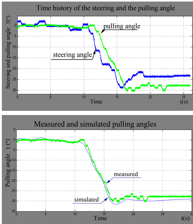
Figure 10 Comparison of measured and simulated pulling angle
