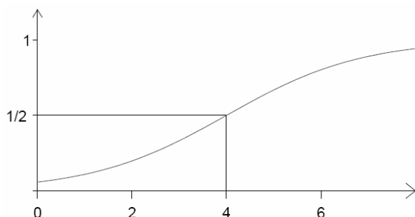
Figure 6 Pliant inequality with \lambda = 0.7 and a = 4 parameters
