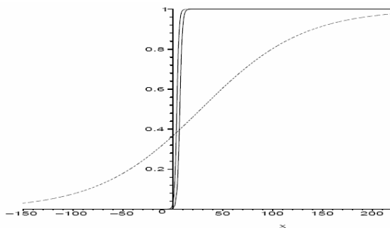
Figure 8 Approximation of pliant multiplication
