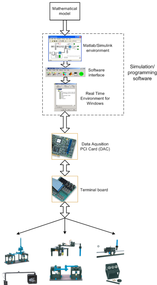
Figure 3 Structure block diagram of development system with different electromechanical models
