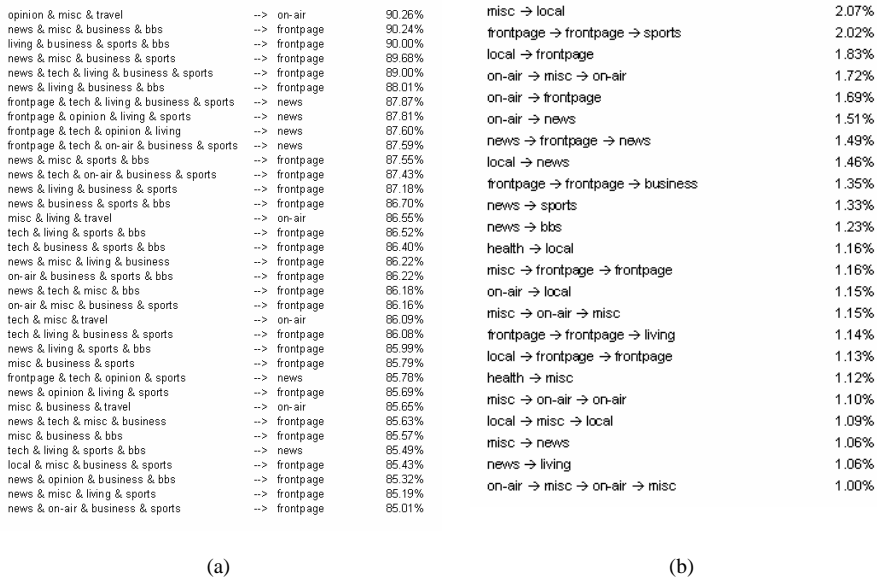
(a) Association rules and (b) sequential rules based on the msnbc.data
