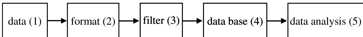
Figure 2: Data preparation
