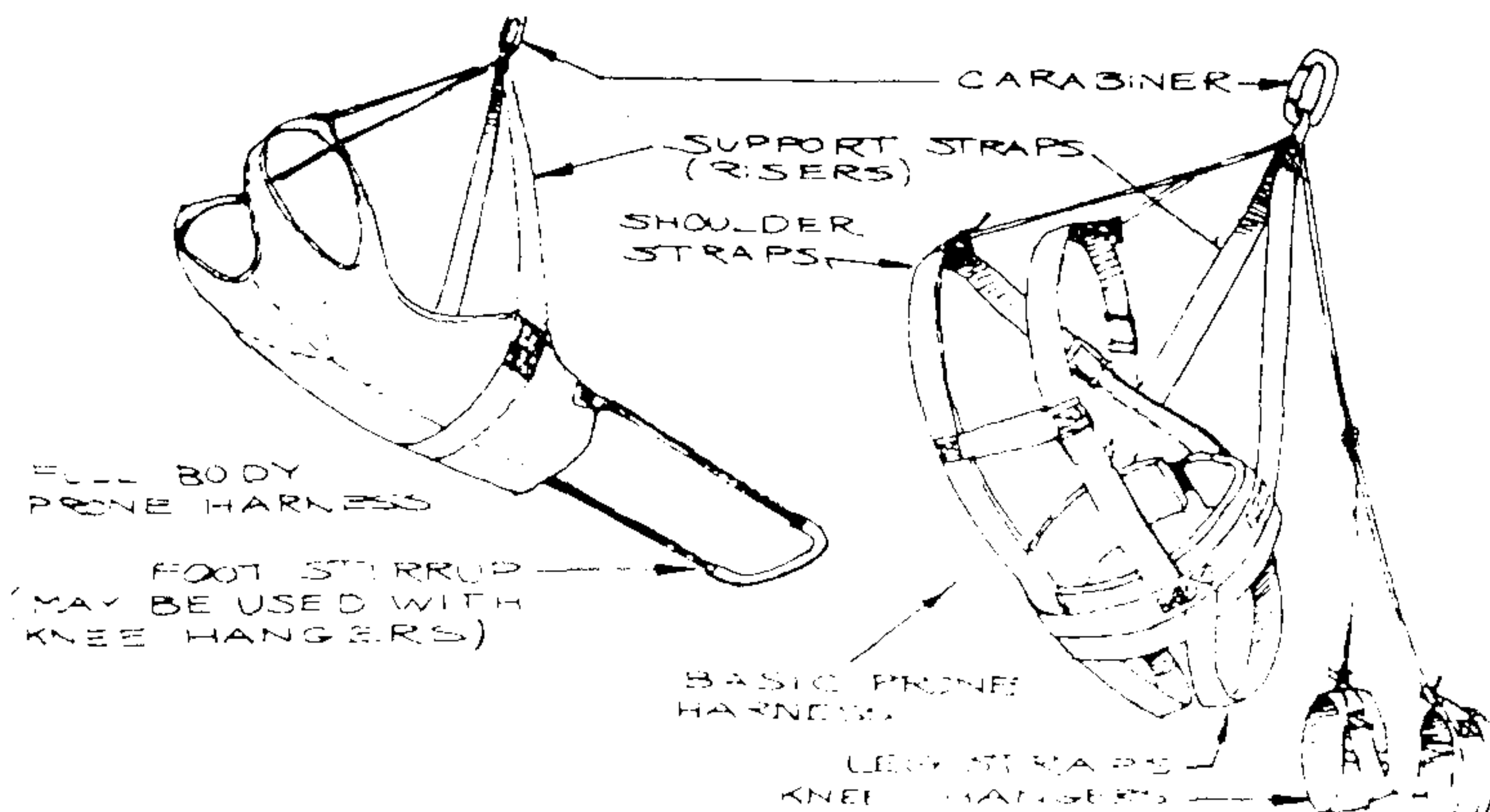
FIGURE 27. - PRONE HARNESSES
